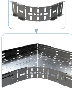
Interior curva
